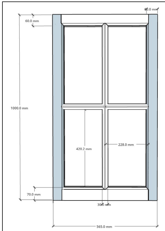
Opening light
