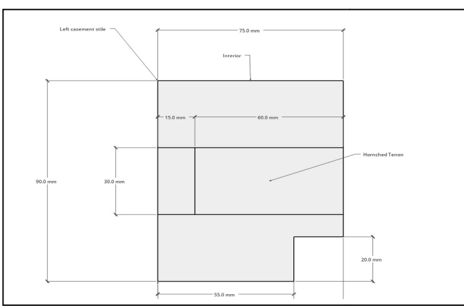
Left Stile top View
