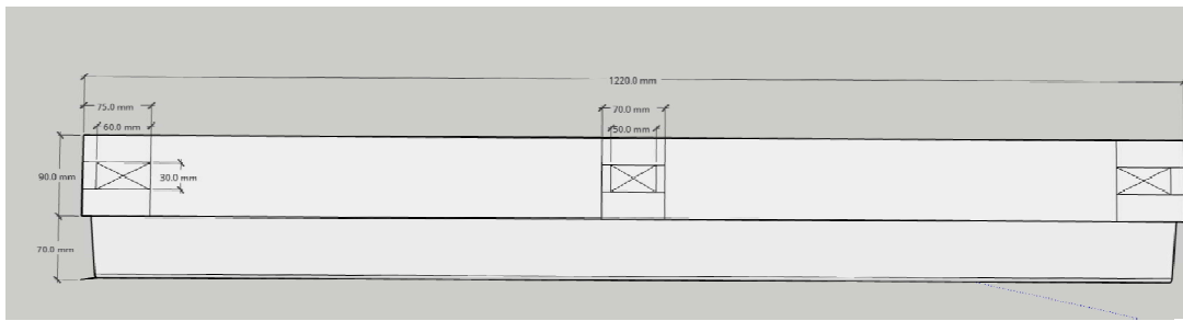
Top View: Mortice positions
